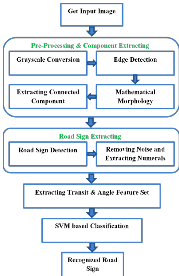
Figure 1: General Diagram of the proposed method
